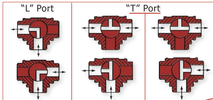
Flow Diagram
