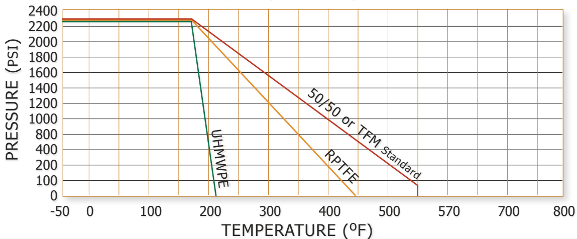
Pressure/Temperature Specifications
