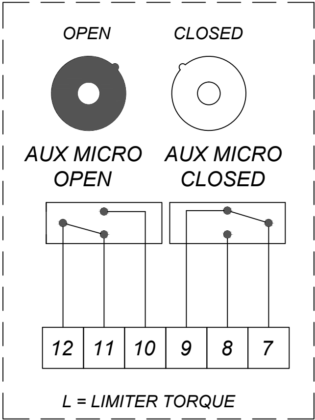
MICRO AUX WITH VALVE IN OPEN POSITION
